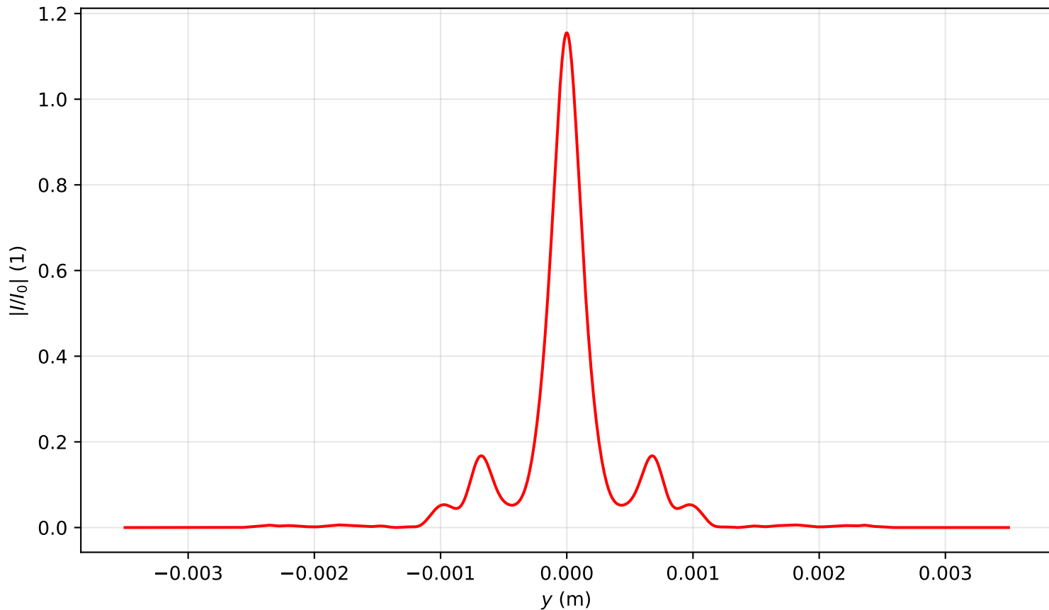
Intensity profile I(x=0, y, z=1.433)/I_0 , P_{in}=8.0P_{cr} , artificial time
